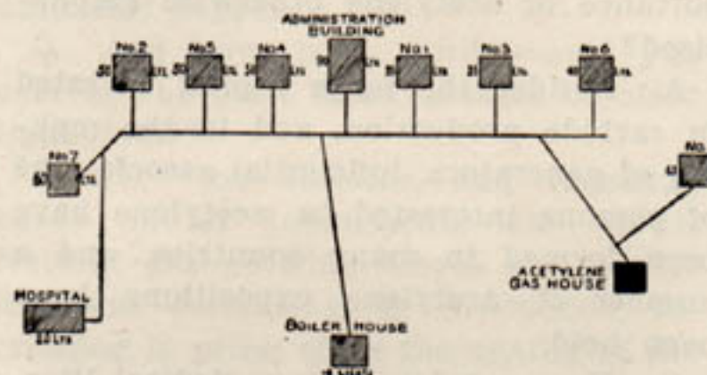
ELEVEN LARGE BUILDINGS OF THE OHIO STATE GIRLS' INDUSTRIAL HOME LIGHTED WITH 600 ACETYLENE JETS FROM ONE GENERATOR.
